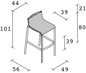
Frame high stool / 41B_O
