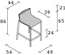
Frame stool / 41A_O
